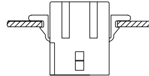
PANEL CUTOUT INFORMATION
