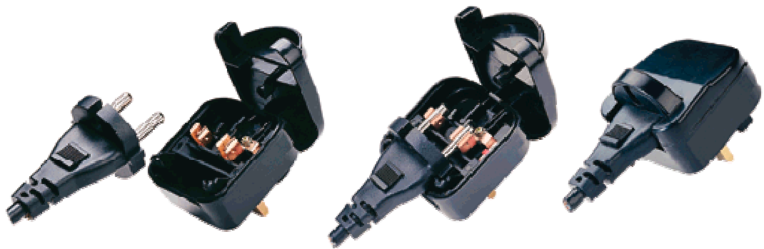
2.5A EUROPLUG NON-EARTHED
