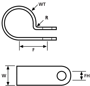
P-Clip H1P-H18P
