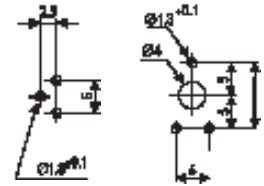
PT10MV top adjust W = 10.3, D = 10.0, H = 4.5 PT10MH side adjust W = 10.3, D = 4.5, H = 12.1
