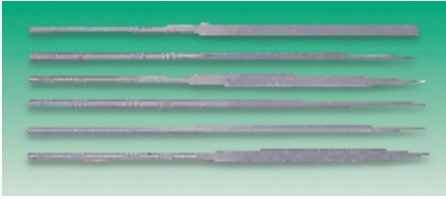
Overall length = 140, blade length = 70, shaft dia = 3.0
