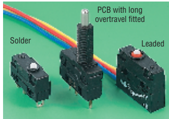
Microswitch: H = 10.2 (unsealed), 16.05 (sealed), W = 6.45, D = 20 Fixing centres = 9.53 Long over travel kit H = 23.95 (from fixing centres) Thread = M6 fine
