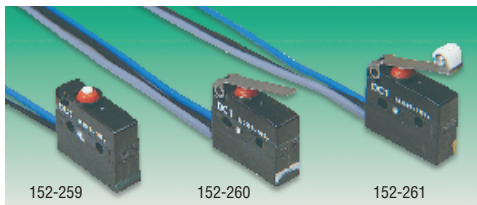
Body H = 15.85, W = 6.5, D = 19.9, Fixing centres = 9.5
