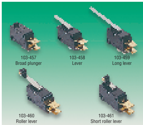
Body: H = 15.9, W = 10.3, D = 27.9, Fixing centres = 22.2 10.3, Quick-connect terminals = 6.35 0.8
