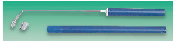
Length without extension = 375. Length with extension = 625. Length (probe) = 225, Dia. (handle) = 17
