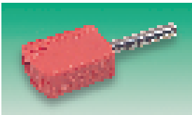
H = 15, W = 8, L = 40 Push to insert/release wire Cage clamp mechanism
