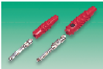
4mm plug L = 51 Plug with 4mm transverse hole L = 59.5
